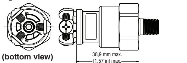
Figure 19. Screw terminal
