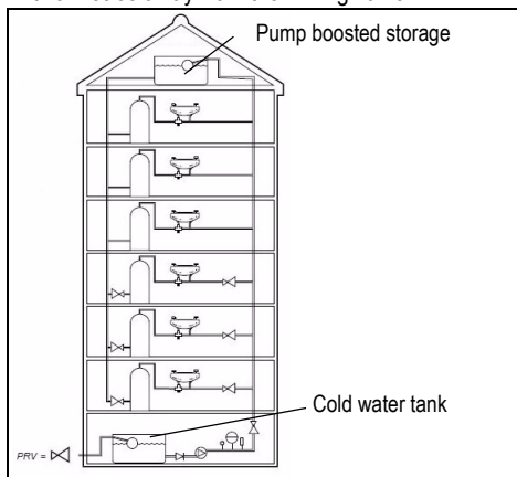
Diagram 6 Multi-storey pump-boostered with high and low storage
