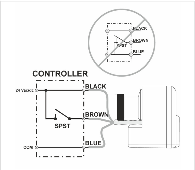
Fig. 2 Electrical wiring M5410C1001
