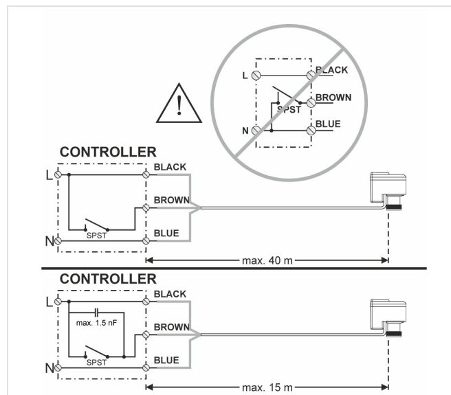
Fig. 1 Electrical wiring M5410L1001
