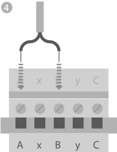
Wire to CS92 Transceiver
