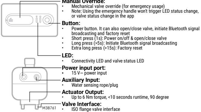
Fig. 2. Components.
