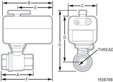
Fig. 7. Dimension diagram.
