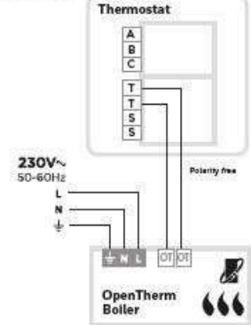
OpenTherm Boiler
